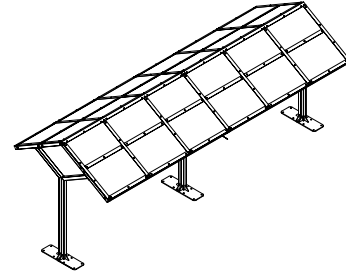
PERSPECTIVE DOUBLE
