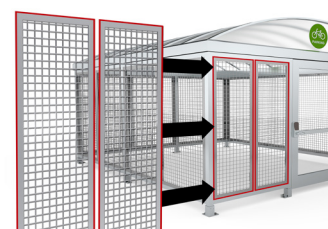
Bike Cage Option (wire grid wall panel detail)
